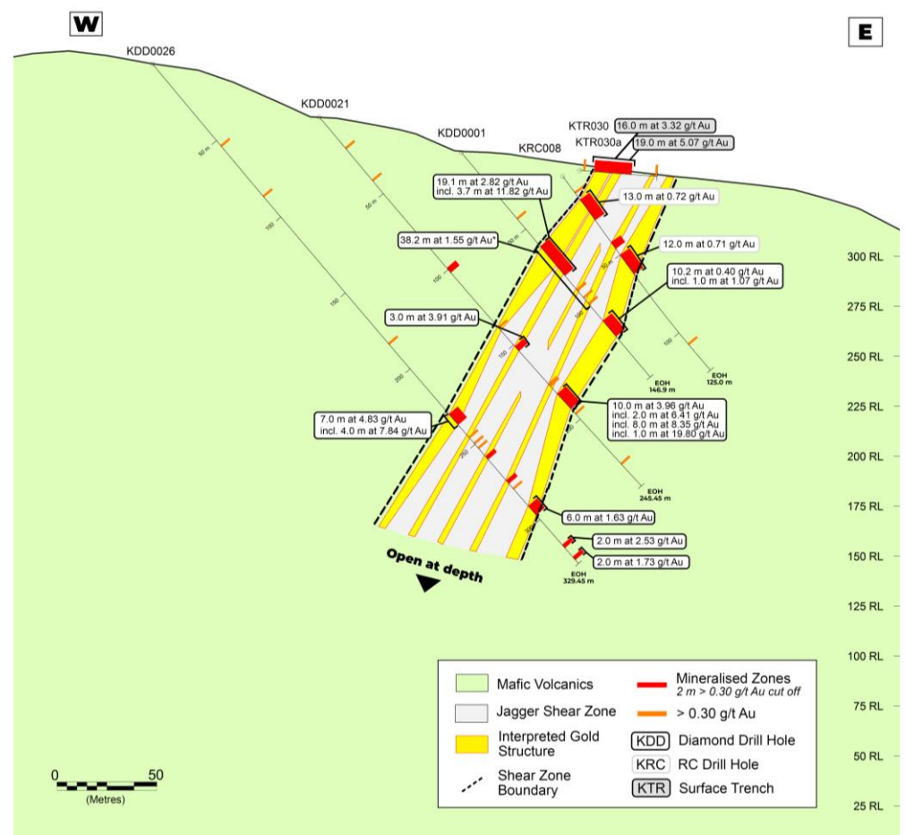
Kossou Gold Project Jagger Zone - Simplified Cross-Section Section JZ 700
