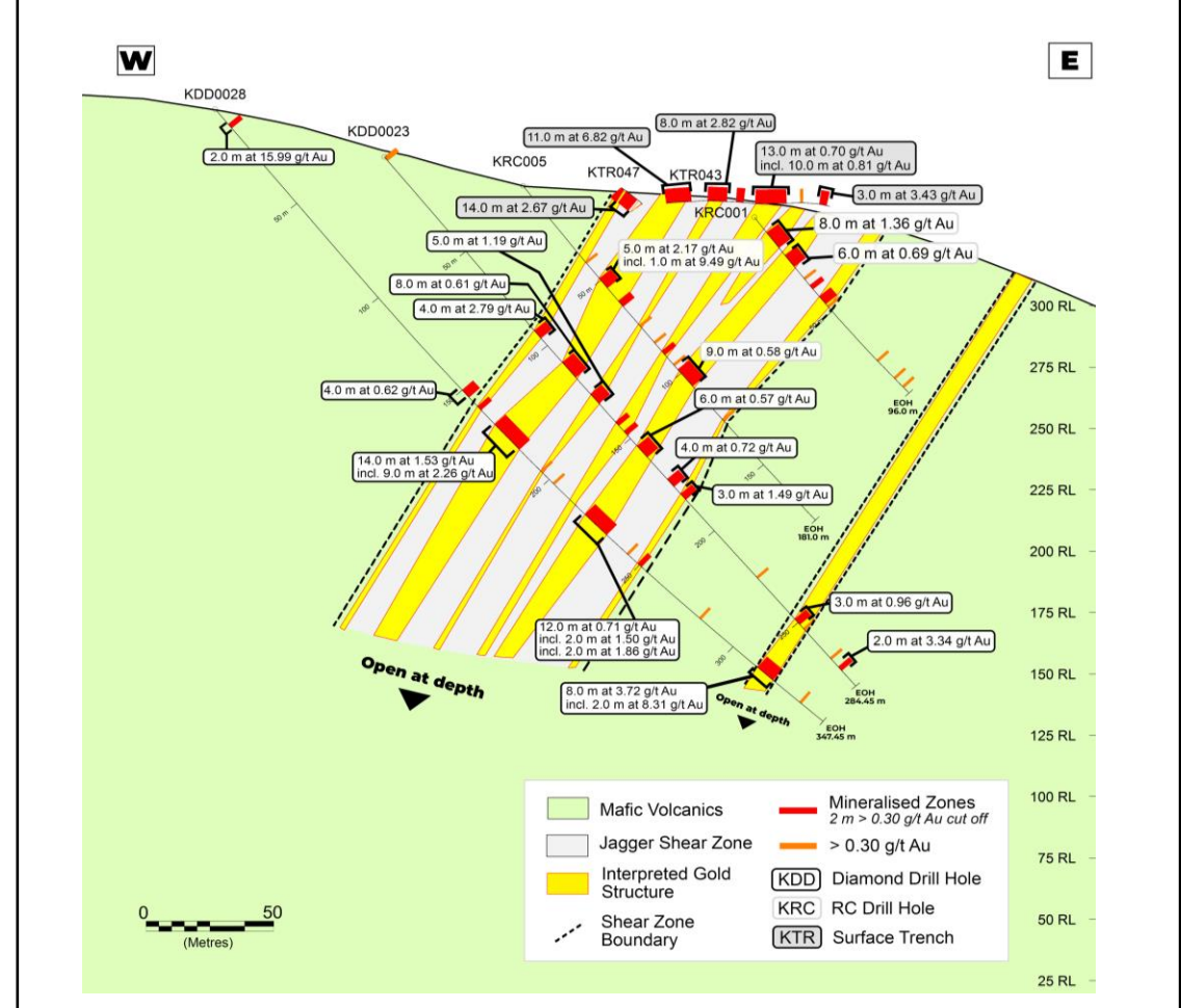
Kossou Gold Project Jagger Zone - Simplified Cross-Section Section JZ 600
